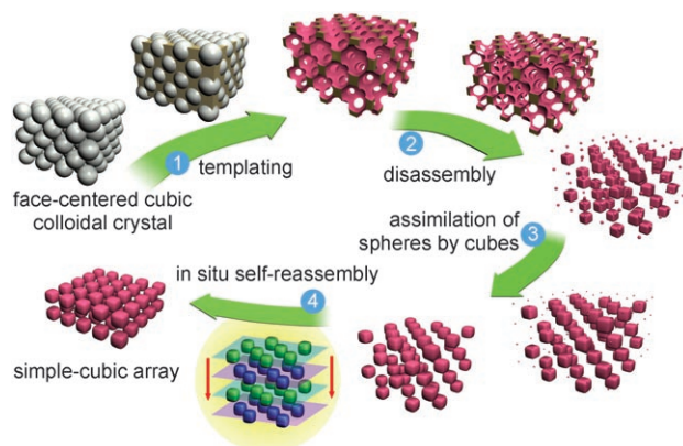
Scheme 1. Schematic of the proposed disassembly and self-reassembly mechanism in situ. A porous skeleton is templated by a face-centered-cubic colloidal crystal and disassembles into its building blocks during calcination. Smaller particles are assimilated by the larger cubes. Alternating layers of cubes merge, driven by capillary forces from a melted phase, producing the observed simple-cubic-packed arrays of nanocubes. For clarity, the interparticle space is exaggerated and any irregular aggregates are ignored.
